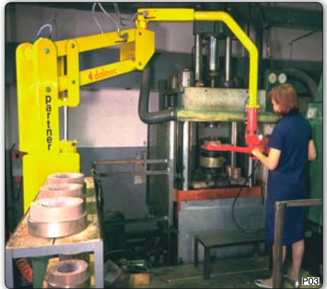
PMC type Partner manipulator, low profile column unit for operating in an area with low ceiling height. The unit is equipped with pneumatic grippers for handling electrical collectors, and enables the operator to handle them in a off-set position. Manipulator Partner PMC, 紧凑型支柱式, 为低房顶厂房而设计。配备气动卡爪, 搬运电气元件。
