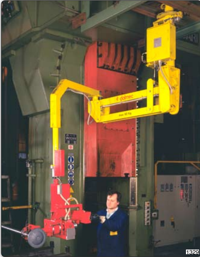
PMF type Partner manipulator, fixed overhead, provided with pneumatic pincer to move with servo-assisted inclination, semi-axes to be transported to the die-stamping machine. Manipulator partner PMF, 悬臂式, 装备气动抓手, 搬运半倾角轴到模具冲压机上。
