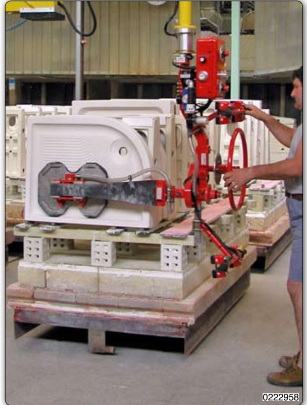
PMF Partner Manipulator, fixed overhead, with suction cups tooling (Venturi) for gripping and manual rotation of shower plates. Manipulator Partner PMF, 悬壁式, 装备文丘里吸盘, 用于抓取和倾斜淋浴板。
