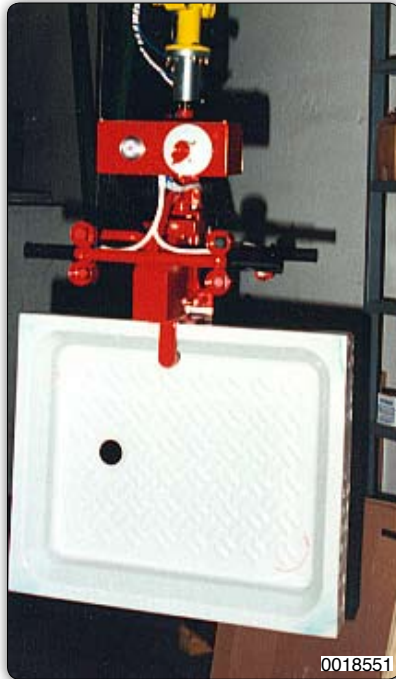
Manipulator with pneumatic tooling for handling shower plates. Manipulator 装备文丘里吸盘, 用于抓取淋浴板。
