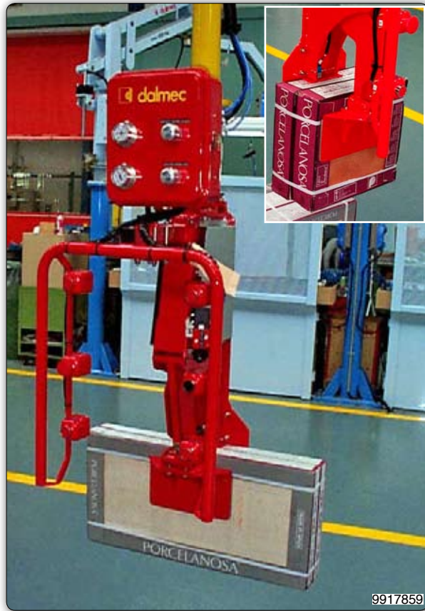
Manipulator with gripper picking system for moving packs of tiles. 装备抓手的机械手臂用于搬运包有瓷砖的木箱。
